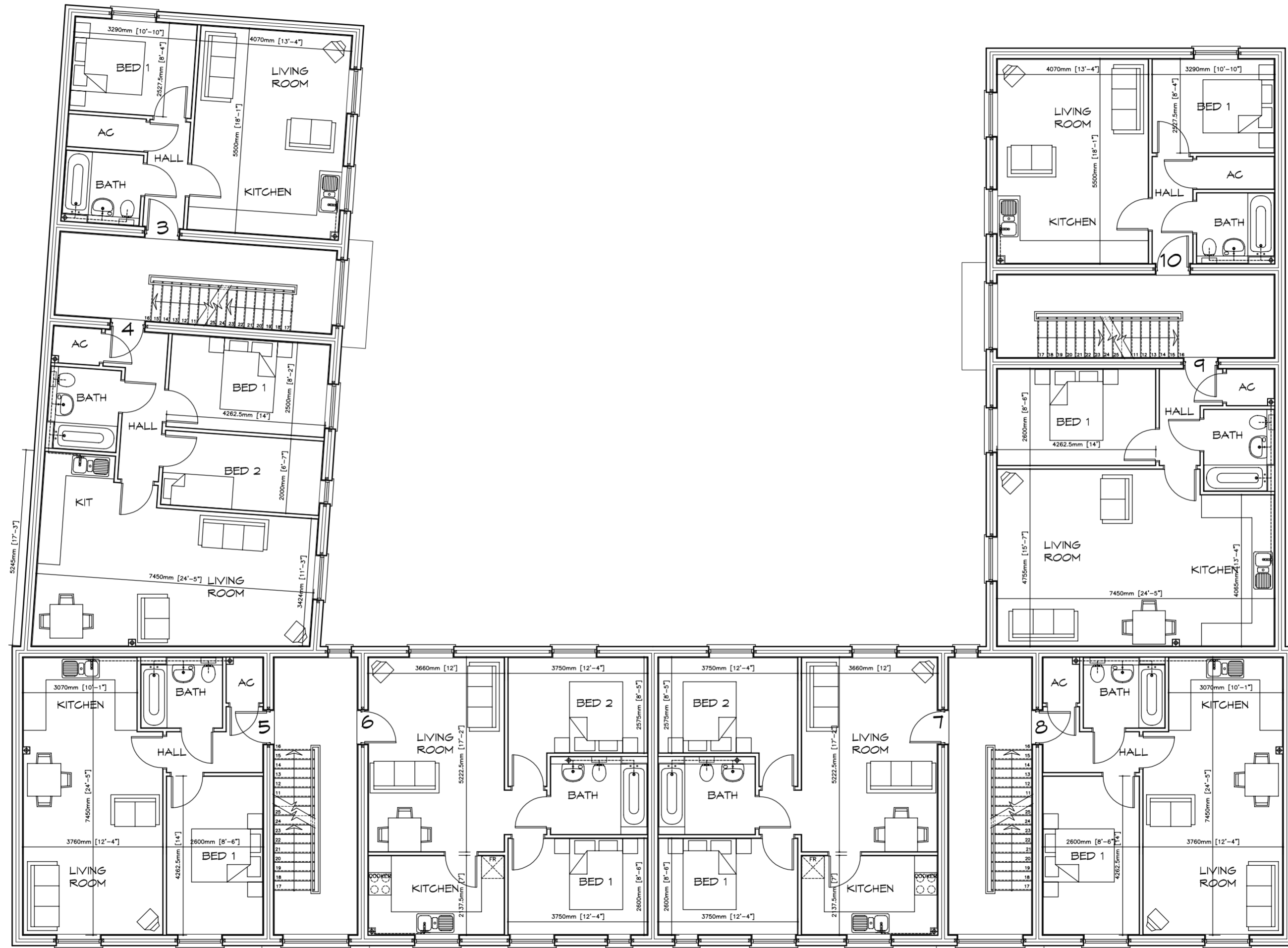
FIRST FLOOR
