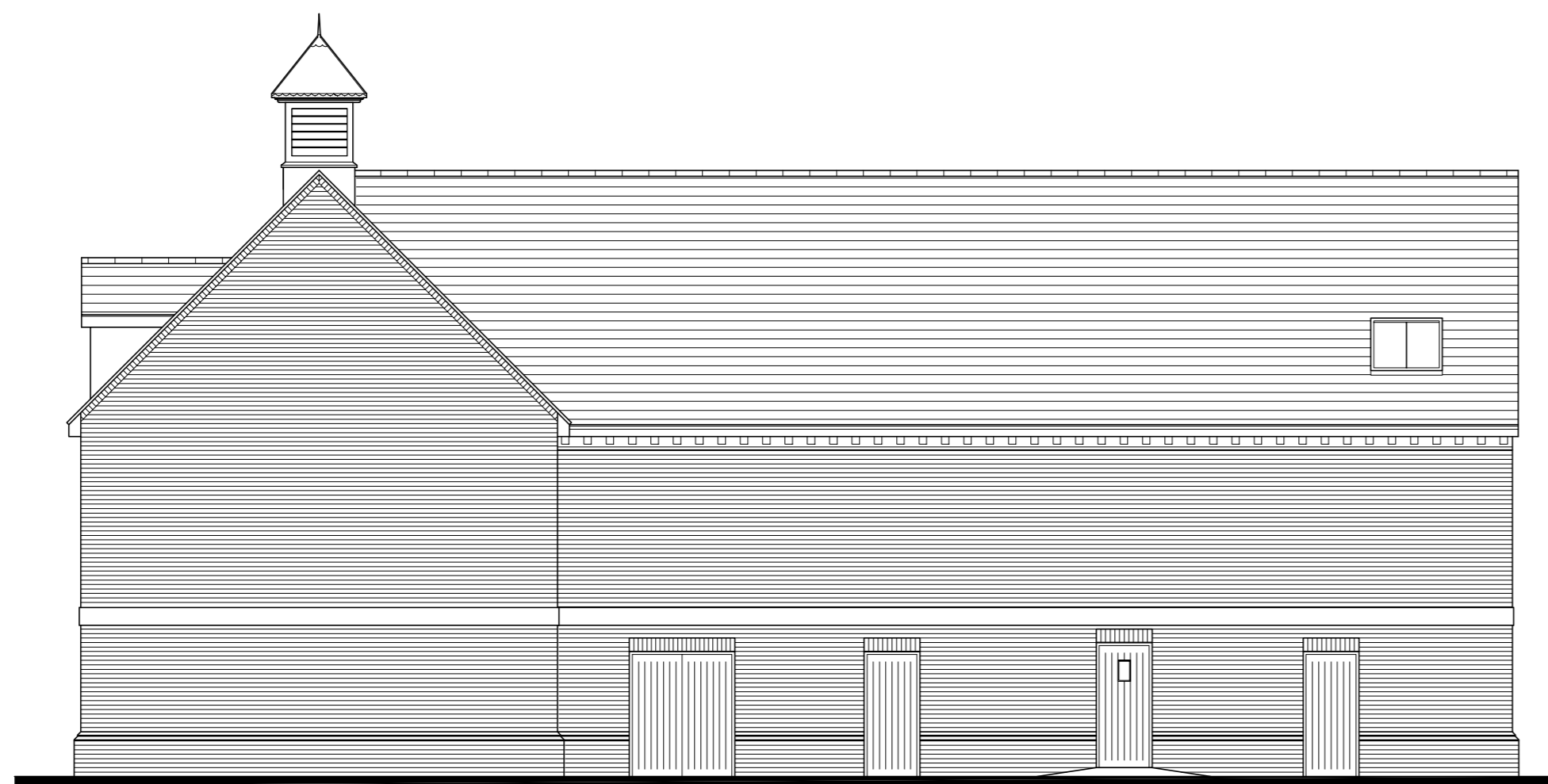
SIDE ELEVATION (TO KITCHINGS HARDWARE AND DIY STORE)
